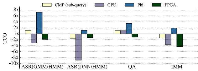
Figure 18: TCO Across Platforms for Each Service
