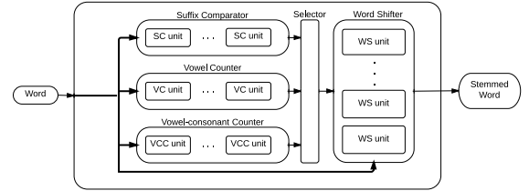
Figure 12: FPGA Stemmer Diagram
