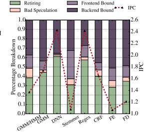
Figure 10: IPC and Bottleneck Breakdown
